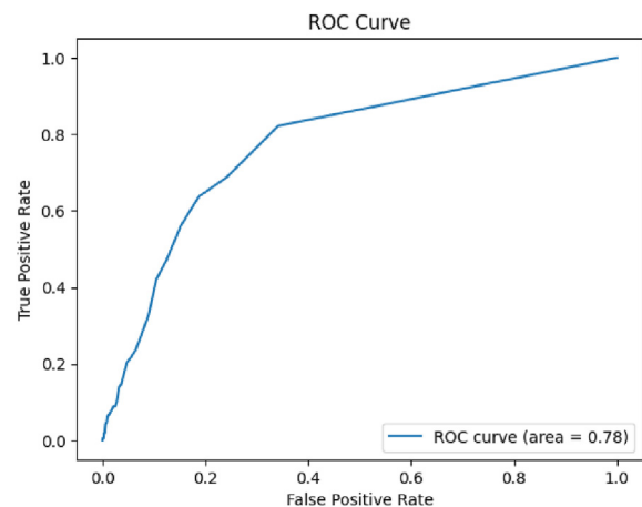
Fig. 8. Roc curve of NN-RF with Smote.
