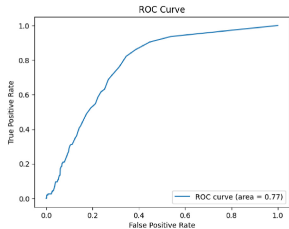
Fig. 7. Roc curve of NN-RF without sampling.
